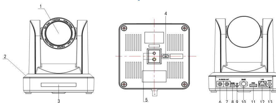
Figure 2.1 Camera Interface
