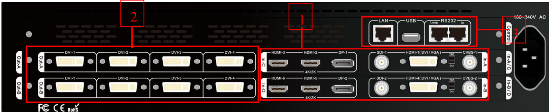
Picture 3-1 Rear panel signal port
