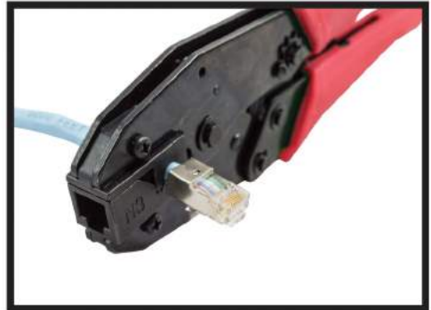
Squeeze the tool to lock the strain relief to hold the cable tightly and grounding
