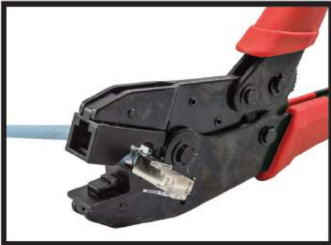
Place the metal strain relief in the right position
