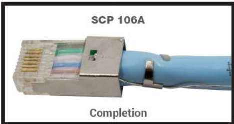
Place the metal strain relief in the right position
